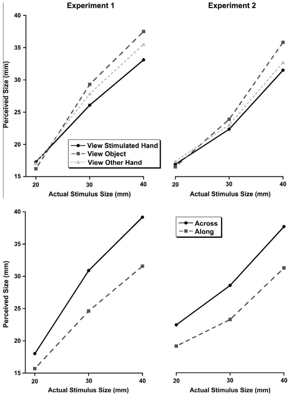
Fig. 3. Mean size judgments. Top panel: perceived size in the two experiments as a function of actual stimulus size and visual context. Bottom panel: perceived size in the two experiments as a function of actual stimulus size and orientation on the hand.
