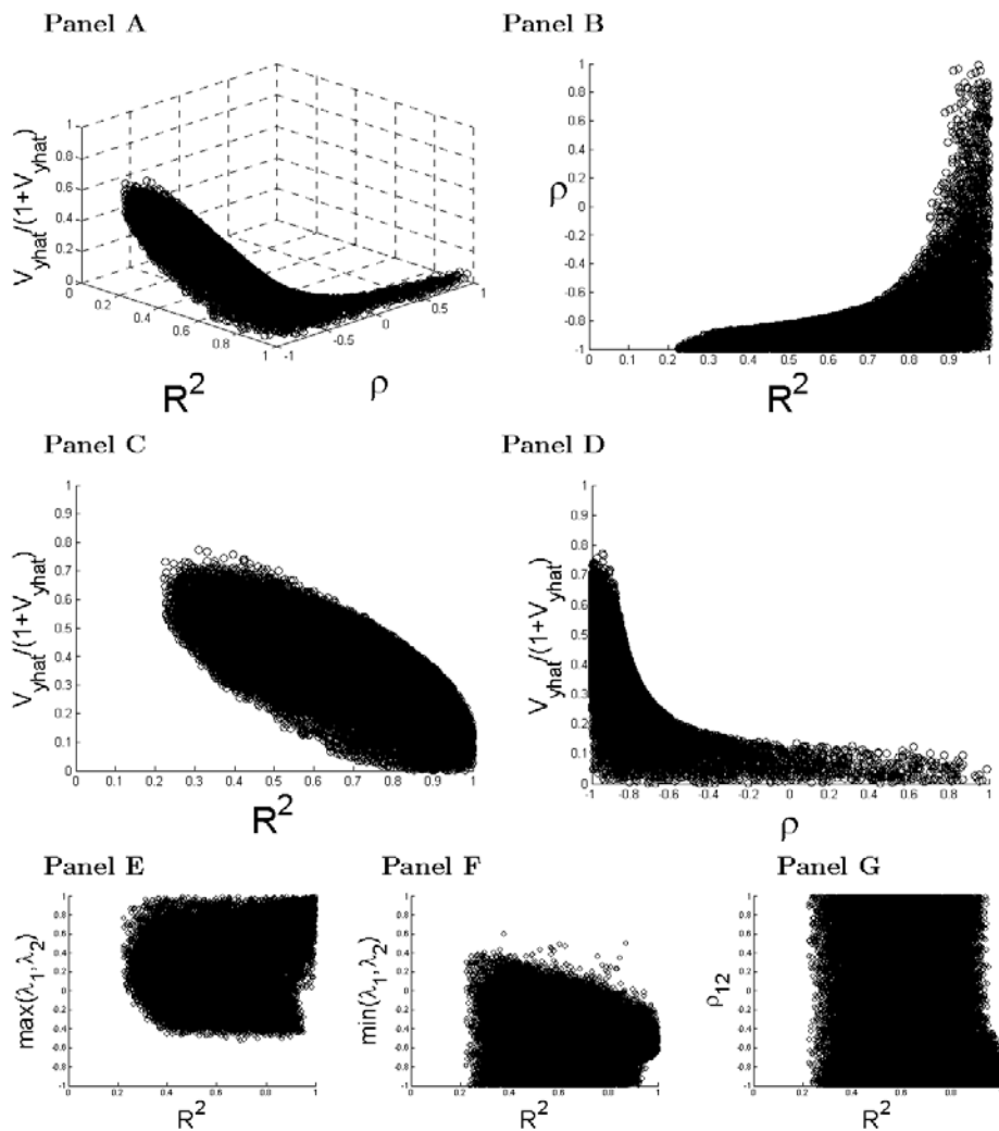
Figure A3. The predictive space \mathbb{P}_U \subset \mathcal{P}_2 for a two predictor model of y_t = \Delta\pi_t , consistent with Stock and Watson's (2007) univariate representation
